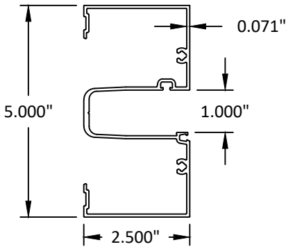
6 HEAD/JAMB
