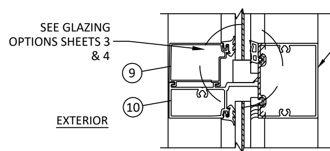
A1 13 VERTICAL SECTION HEAD - CONCRETE/MASONRY W/ 1X BUCK MEDIUM/HEAVY CONFIGURATION
