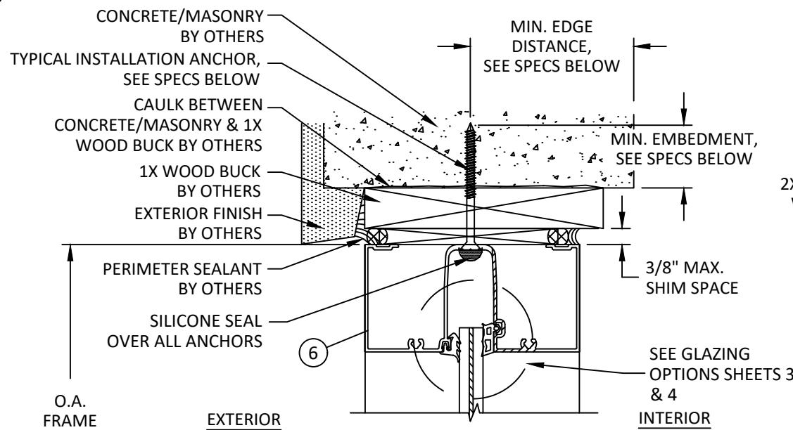
A 12 VERTICAL SECTION HEAD - CONCRETE/MASONRY W/ 1X BUCK LIGHT CONFIGURATION
