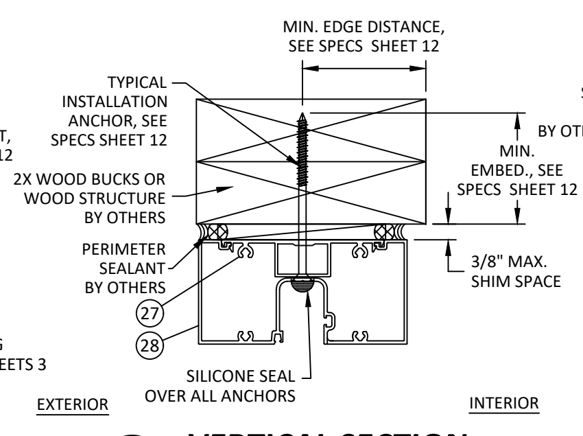
D1 13 VERTICAL SECTION HEAD - WOOD FRAMING MEDIUM/HEAVY CONFIG. - TYP. INSTALLATION
