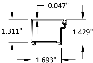
9 GLASS STOP
