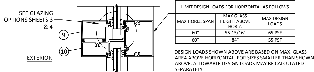
A 12 VERTICAL SECTION HEAD - CONCRETE/MASONRY W/ 1X BUCK LIGHT CONFIGURATION
