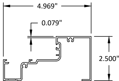
11 SILL (UP TO ± 50 PSF)
