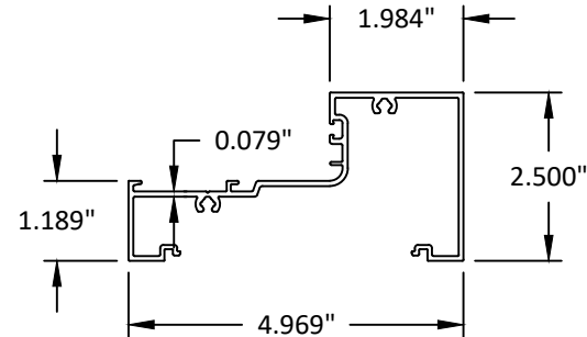
25 SILL (UP TO +70/-90 PSF)
