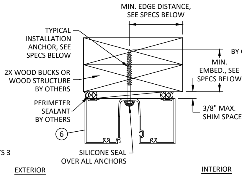
D 12 VERTICAL SECTION HEAD - WOOD FRAMING LIGHT CONFIG. - TYPICAL INSTALLATION
