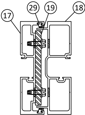
EXPANSION MULLION
