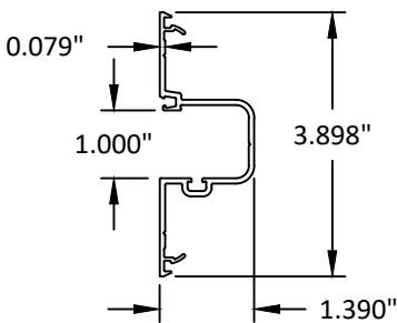
4 DEEP POCKET FILLER
