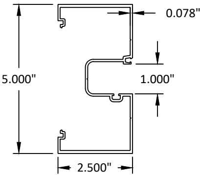
1 JAMB/VERTICAL
