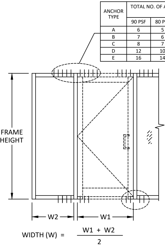
SINGLE DOOR
