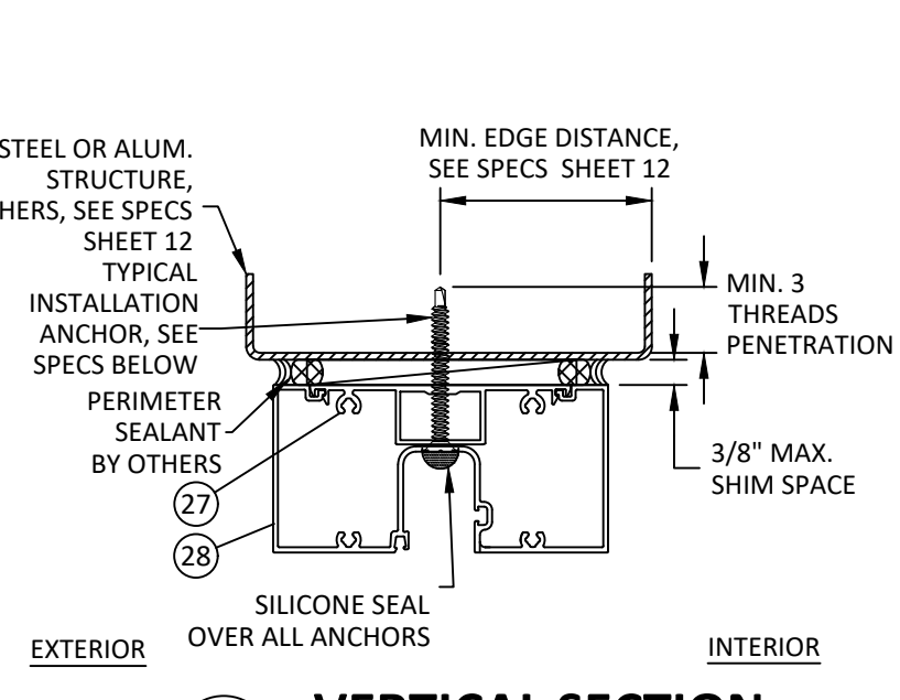
E1 13 VERTICAL SECTION HEAD - METAL SUBSTRATE MEDIUM/HEAVY CONFIG. - TYP. INSTALLATION
